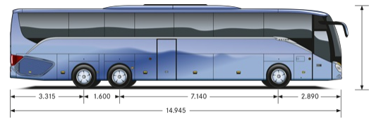
Alle maten in millimeters.
